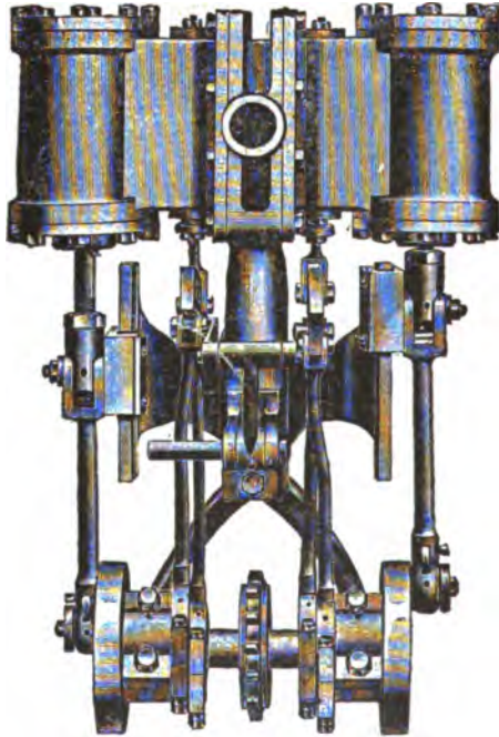
FIG. 258.—The "Eastman" Steam Carriage Engine.
